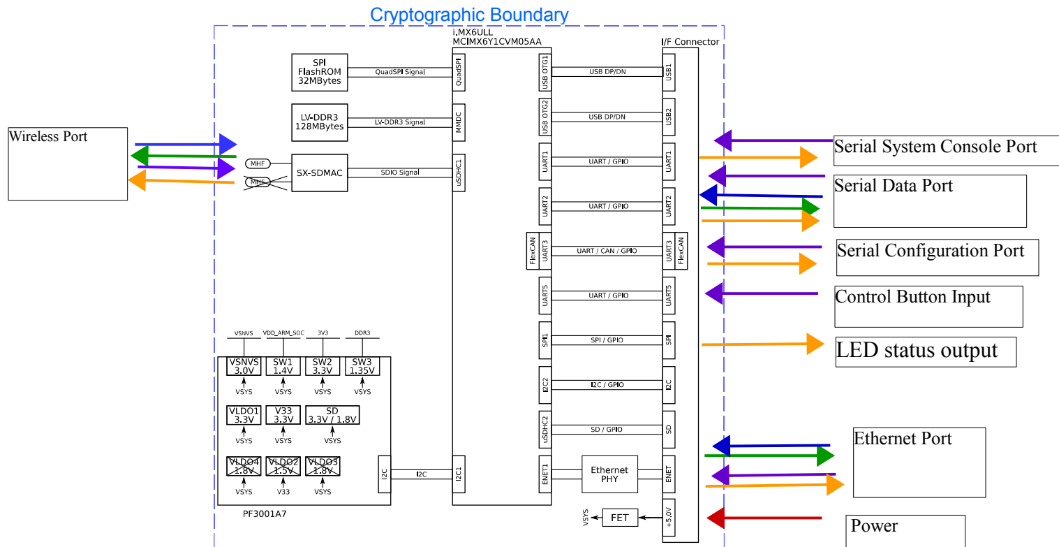
Figure 3 - SX-590-1402 Cryptographic Module Block Diagram
