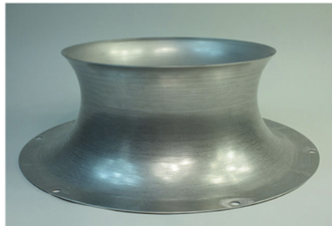
Aluminum inlet for the Commercial HVAC industry. 0.060" thick aluminum 20.00" diameter X 8.00" height formed on a CNC spinning lathe.
