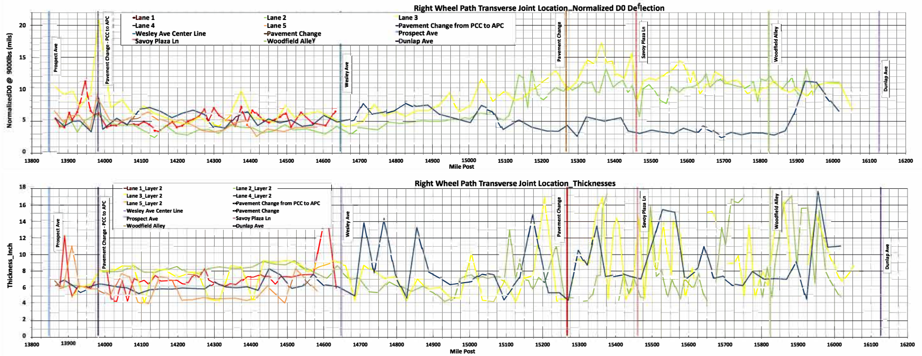
MAXIMUM DEFLECTION DATA (D0) AND GPR THICKNESS PROFILES AT TRANSVERSE JOINT LOCATIONS
