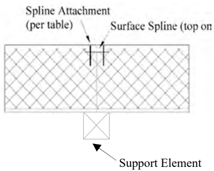
FIGURE 3A—INTERIOR SUPPORT SPLINE
