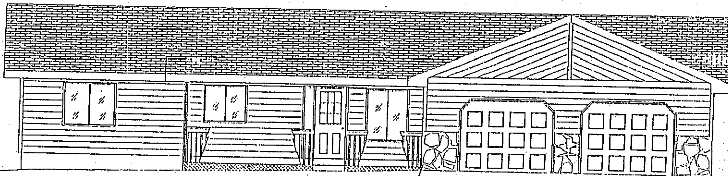
Front Elevation
