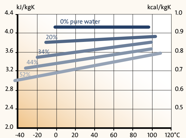
Fig. 2.2.18: Heat capacity vs. temperature for ethylene glycol
