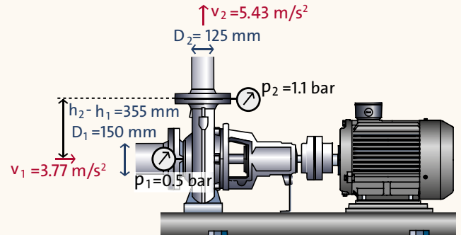
Fig. 2.2.7: Standard end-suction pump with different dimensions of suction and discharge ports (Example)
