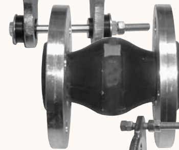
Fig. 2.1.13: Rubber bellows expansion joints without tie bars
