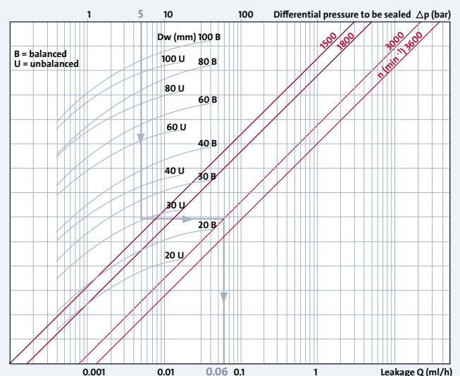
Fig. 1.3.21: Leakage rates
