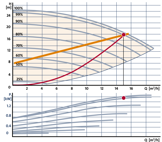
Fig. 4.4.5: A speed-controlled pump in a closed system
