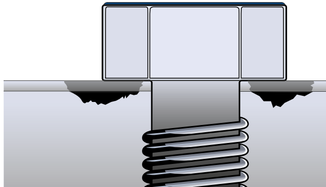
Fig. 1.6.5: Crevice corrosion
