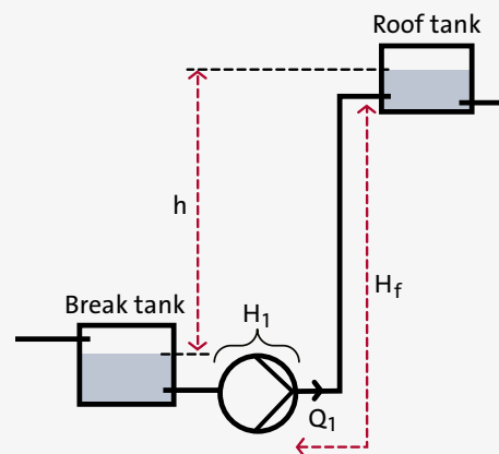
Fig. 3.1.6: Open system with positive geodetic lift
