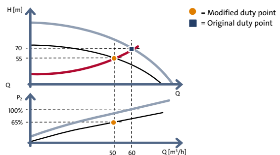
Fig. 4.1.13: Relative power consumption - speed control
