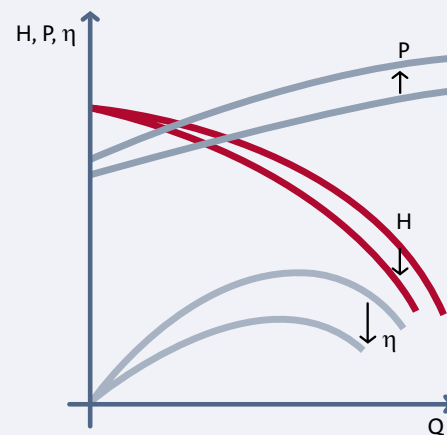
Fig. 1.5.2: Changed head, efficiency and power input for liquid with higher viscosity
