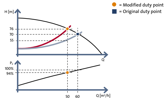
Fig. 4.1.10: Relative power consumption - throttle control
