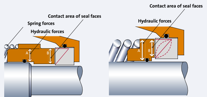
Fig. 1.3.6: Interaction of forces on the balanced shaft seal
