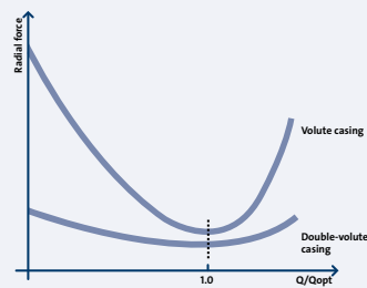
Fig. 1.1.18: Single-volute casing Double-volute casing
