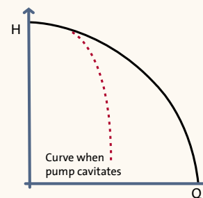
Fig.: 2.2.11: Pump curve when pump cavitates
