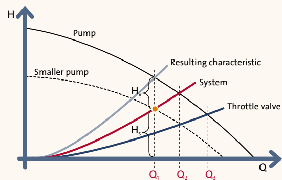
Fig.: 4.1.2: The throttle valve increases the resistance in the system and consequently reduces the flow.
