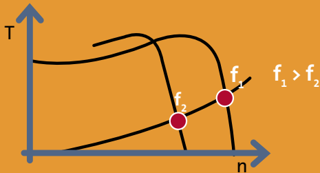
Fig. 4.5.1: Displacement of motor torque characteristic
