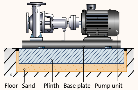
Fig. 2.1.8: Floating plinth
