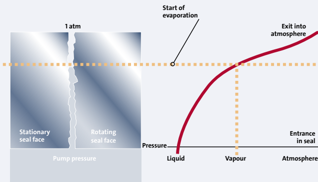
Fig. 1.3.5: Optimum ratio between fine lubrication properties and limited leakage
