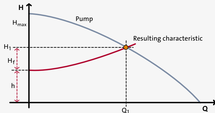
Fig. 3.1.7: System characteristic together with the pump performance curve for the open system in figure 3.1.6
