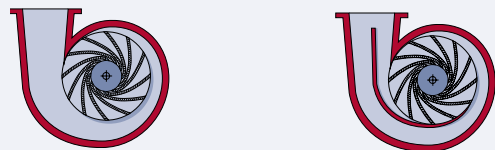
Fig. 1.1.18: Single-volute casing Double-volute casing
