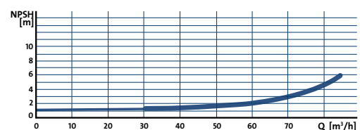
Fig. 1.1.9: The NPSH-curve of a typical centrifugal pump
