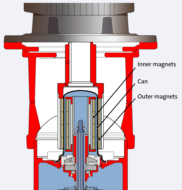
Fig. 1.2.9: Magnetic-driven multistage pump
