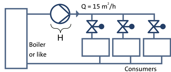
Fig. 4.4.4: Closed system
