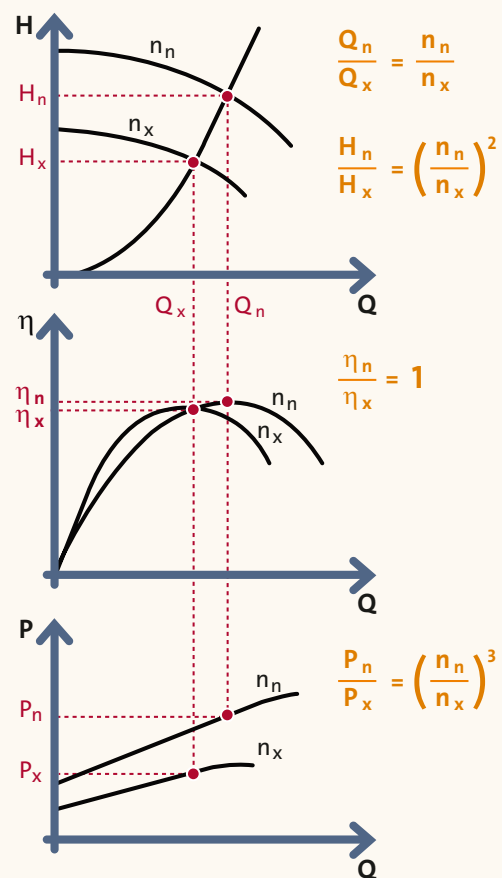
Fig. 4.1.5: Pump parameters for different affinity equations
