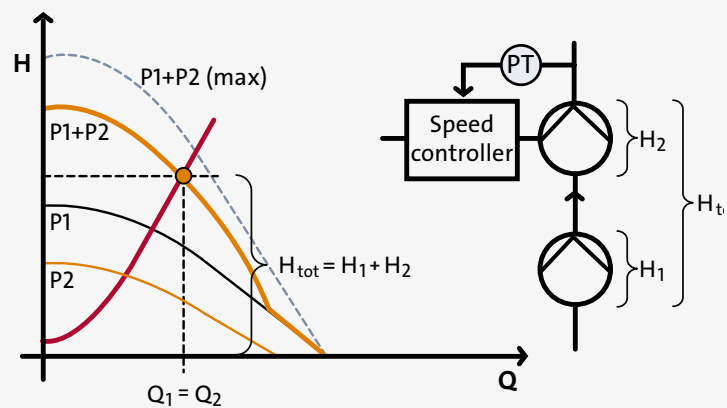
Fig. 3.2.7: Equal sized fixed speed pump and speed-controlled pump connected in series. A pressure transmitter PT together with a speed controller is making sure that the pressure is constant at the outlet of P2.
