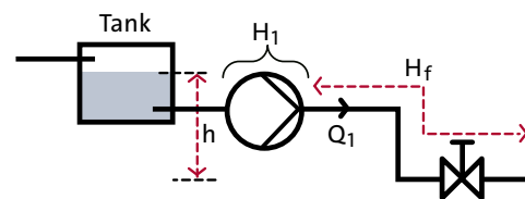
Fig. 3.1.8: Open system with negative geodetic lift
