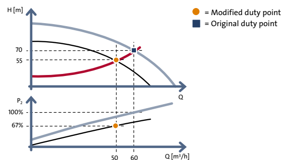
Fig. 4.1.12: Relative power consumption - modifying impeller diameter
