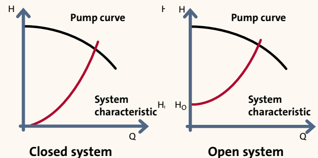
Fig 4.4.3: System characteristic point of a closed and an open system
