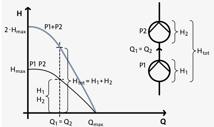
Fig. 3.2.5: Two equal sized pumps connected in series
