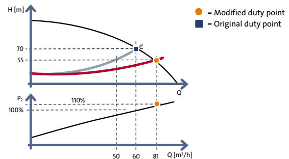
Fig. 4.1.11: Relative power consumption - bypass control
