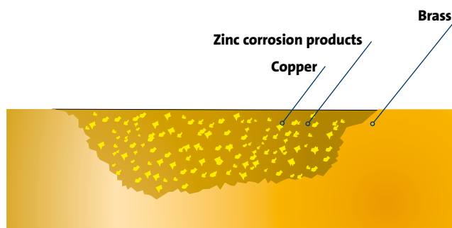
Fig. 1.6.7: Selective corrosion
