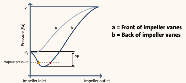
Fig.: 2.2.10: Development of pressure through a centrifugal pump
