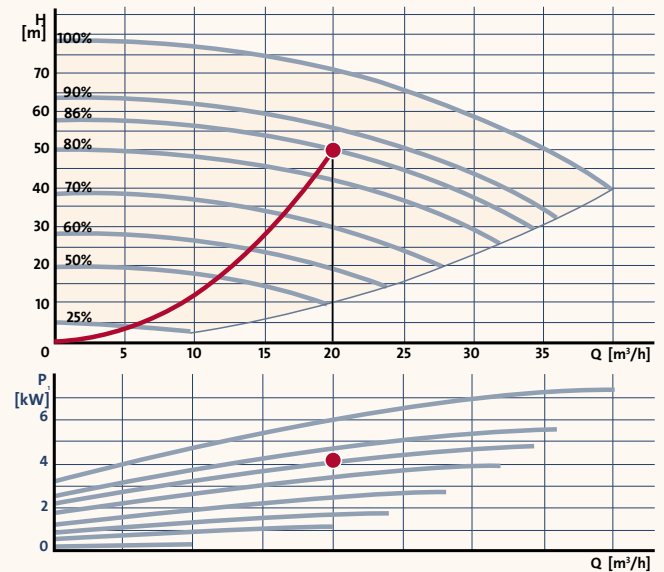
Fig 4.4.2: Performance curve for a speed-controlled pump
