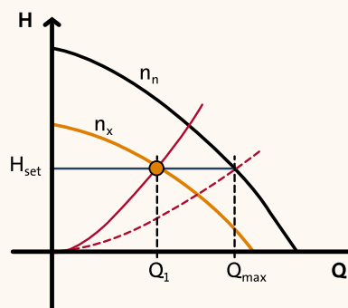
Fig. 4.2.3: Heating system with speed-controlled circulator pump delivering constant differential pressure to the system
