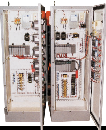
PLC-Based Chemical Feeder System
