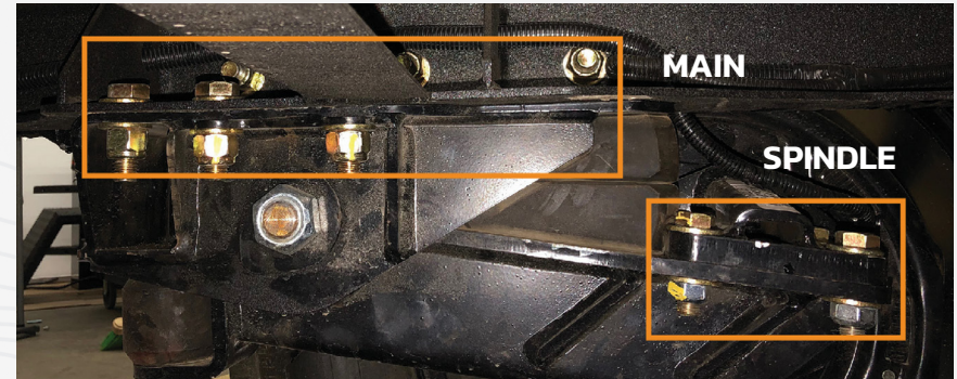
Fig 7.1 Suspension
