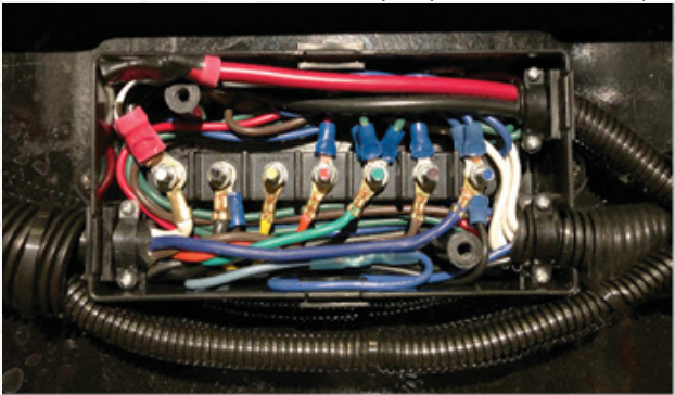
Fig 5.4 Electrical
