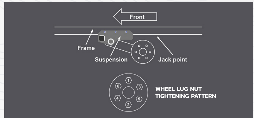
Fig 7.2 Suspension
