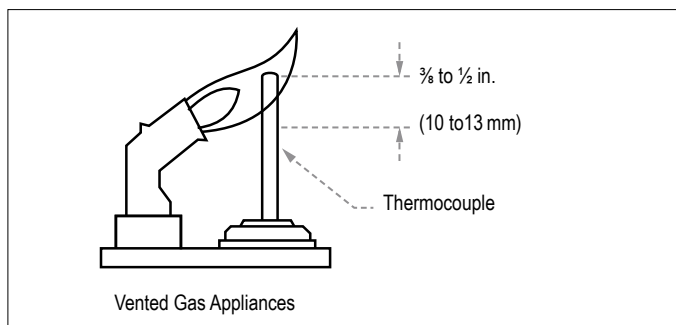
Figure 15: Proper Flame Impingement on Thermocouple
