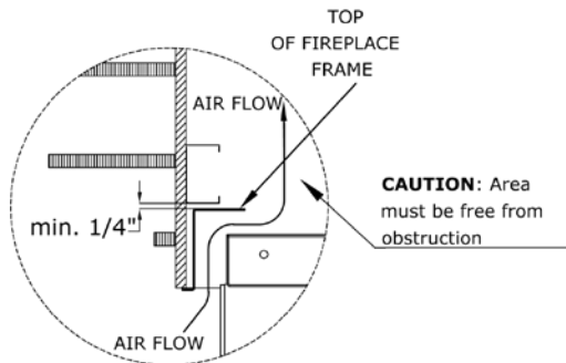
Section Detail View B-B
