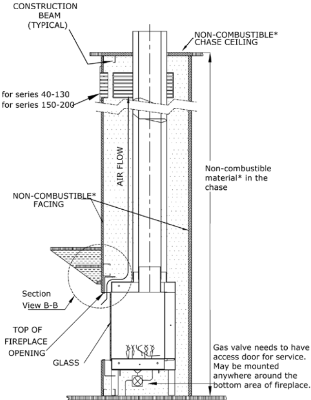
SECTION VIEW B
