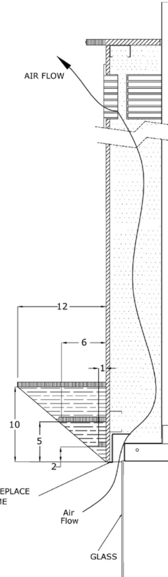
SECTION DETAIL VIEW B-1B
