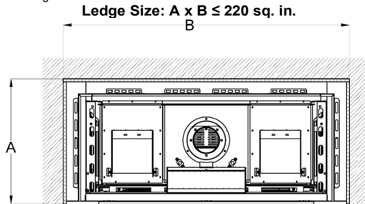
A = ledge depth, B= ledge length (Top View)
