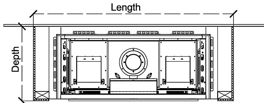
Fireplace Chase (Top View)
