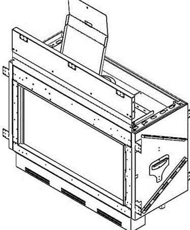
Zero-Clearance Stand-Offs (Isometric View)
