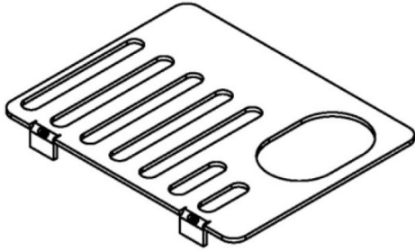
Left grill cover (BL110DW002)
