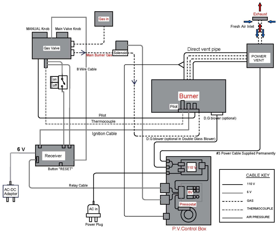
Power Vent System Wiring Diagram
