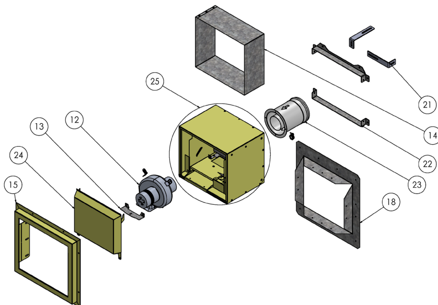
Flush Horizontal Termination Power Vent Fan Box Components
