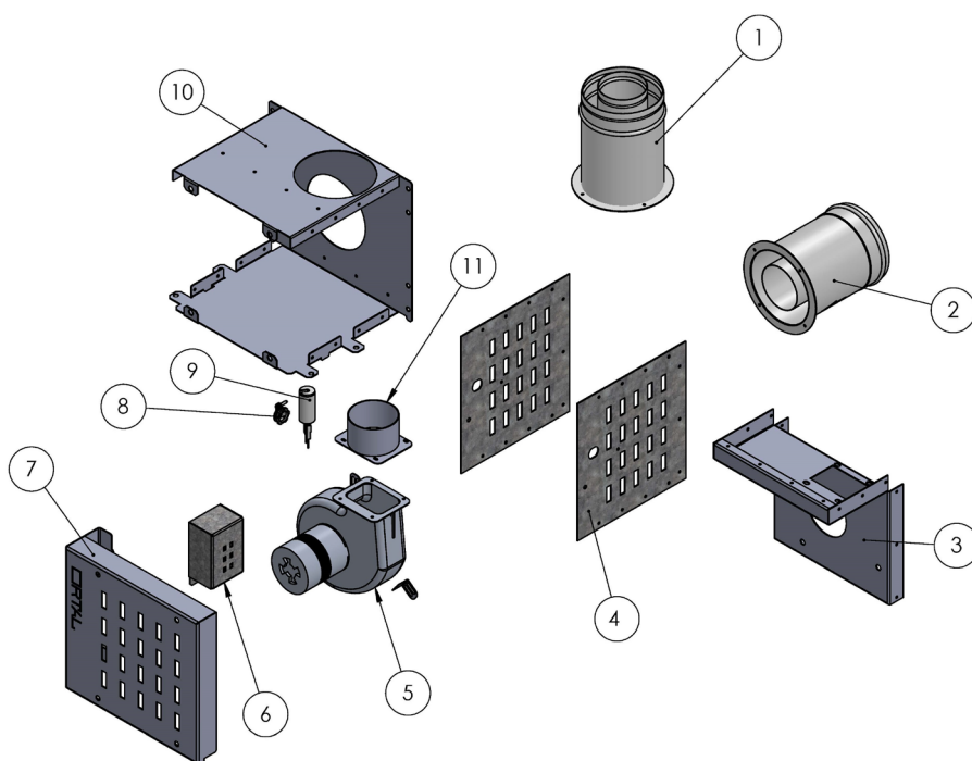
Inline-90 Power Vent Fan Box Components
