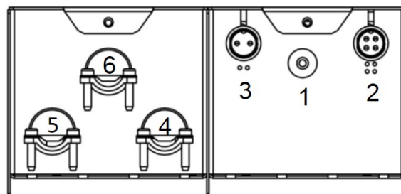
Wire Connection for Power Vent Control Box
