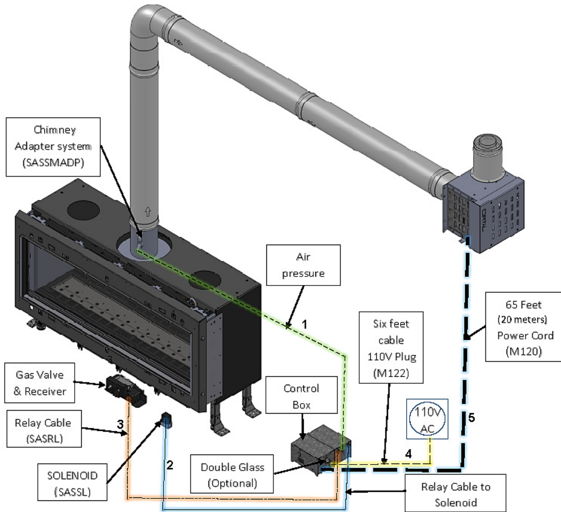
Wire Connection for Power Vent
