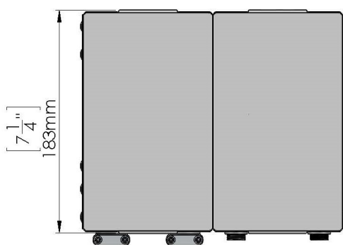
Dimensions for Power Vent Control Box
