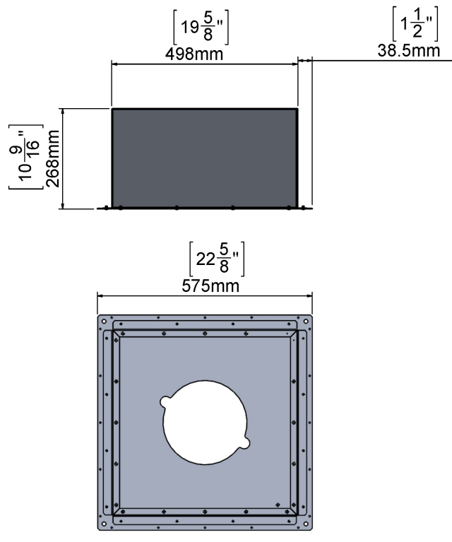
Dimensions for Vertical Termination Power Vent Riser
