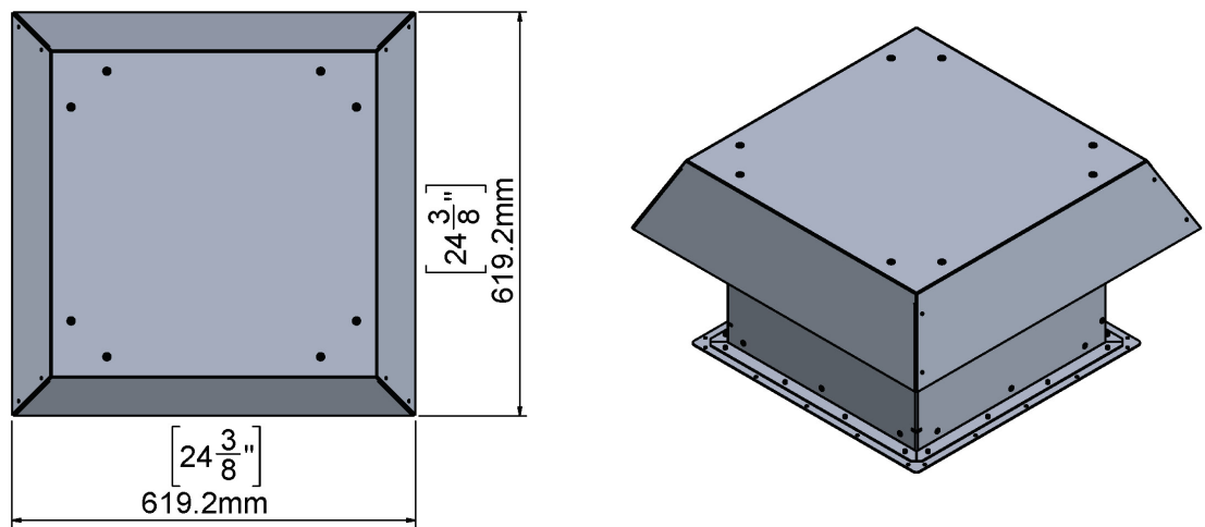
Dimensions for Vertical Termination Power Vent
