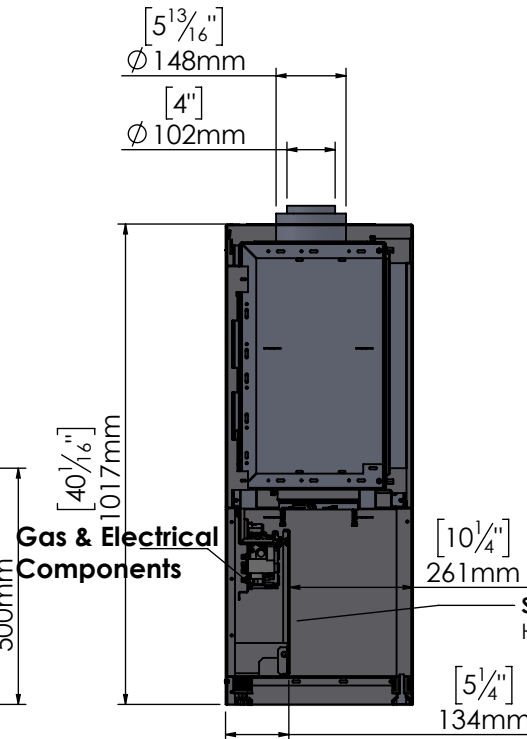
Left Side Section View
