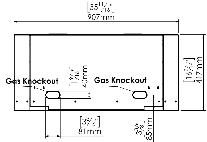
Back View
