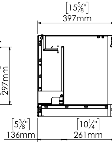
Left Side Section View
