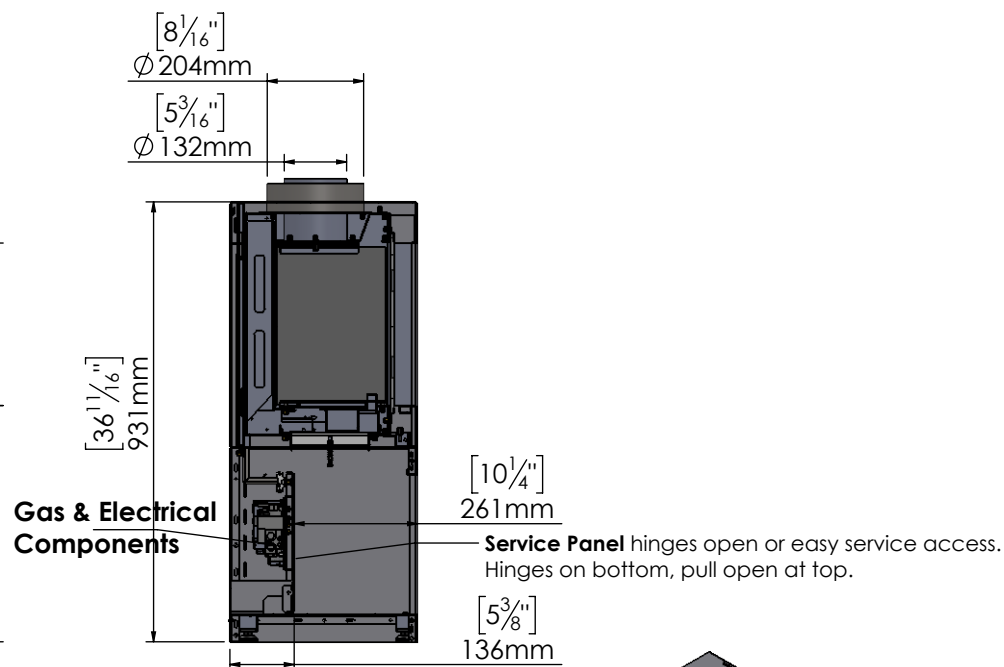
Left Side Section View
