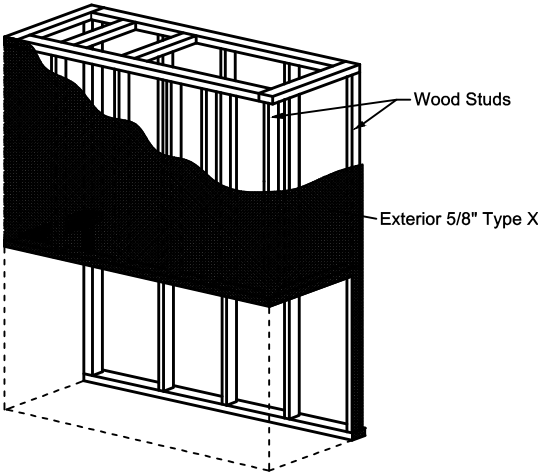
\frac{5}{8} " Type X Drywall Placement
