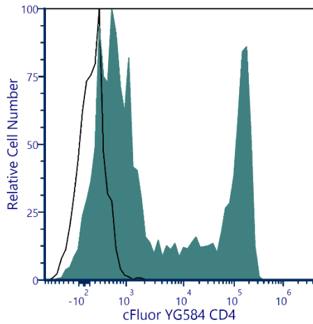
Human peripheral lymphocytes stained with cFluor™ YG584 CD4 (clone SK3) (filled histogram) or mouse cFluor™ YG584 IgG1, κ isotype control (open histogram).
