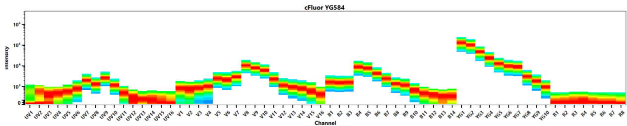
Spectral signature of cFluor™ YG584 from a Cytex® Aurora 5 laser system.
