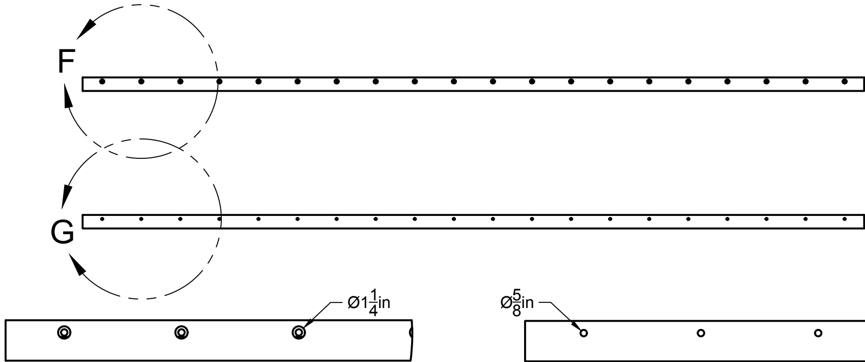
DETAIL F SCALE 1:10
