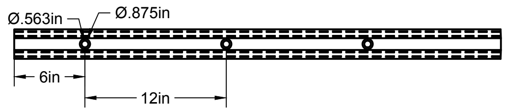
DETAIL A SCALE 1:8
