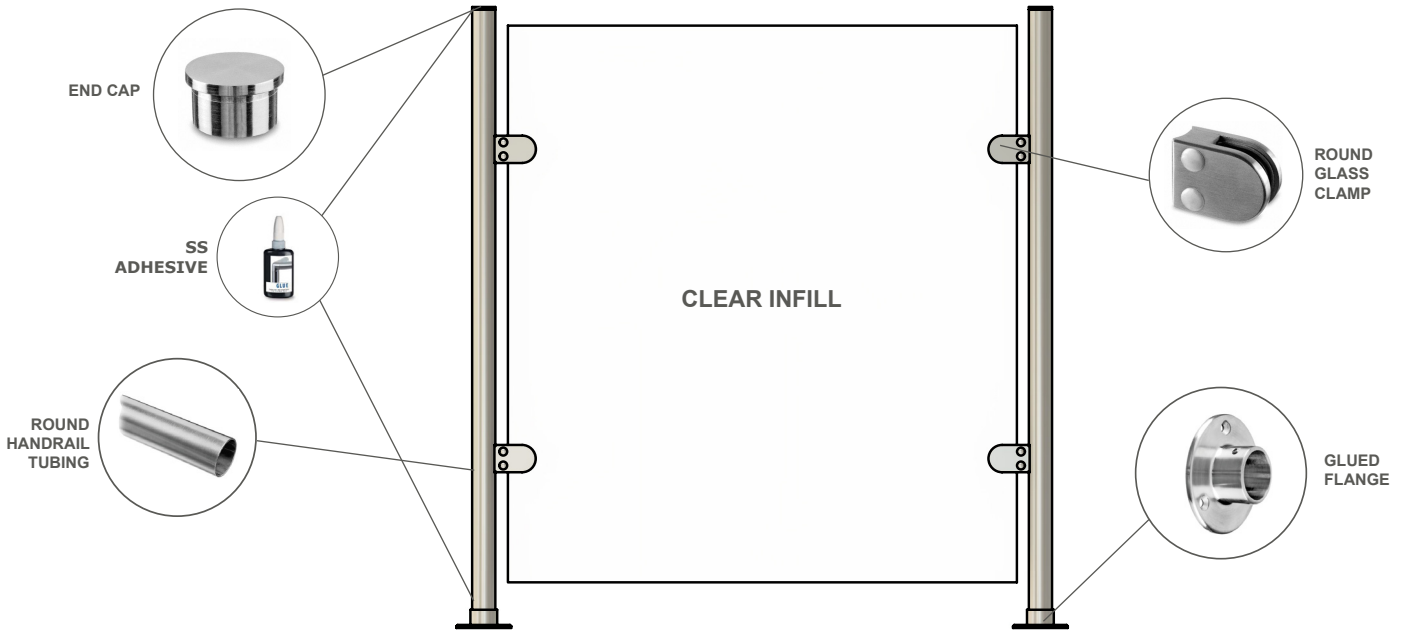
END CAP (2) Ø1.5" GLUED CAP FOR TOP OF POSTS
